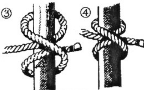
CLOVE HITCH
